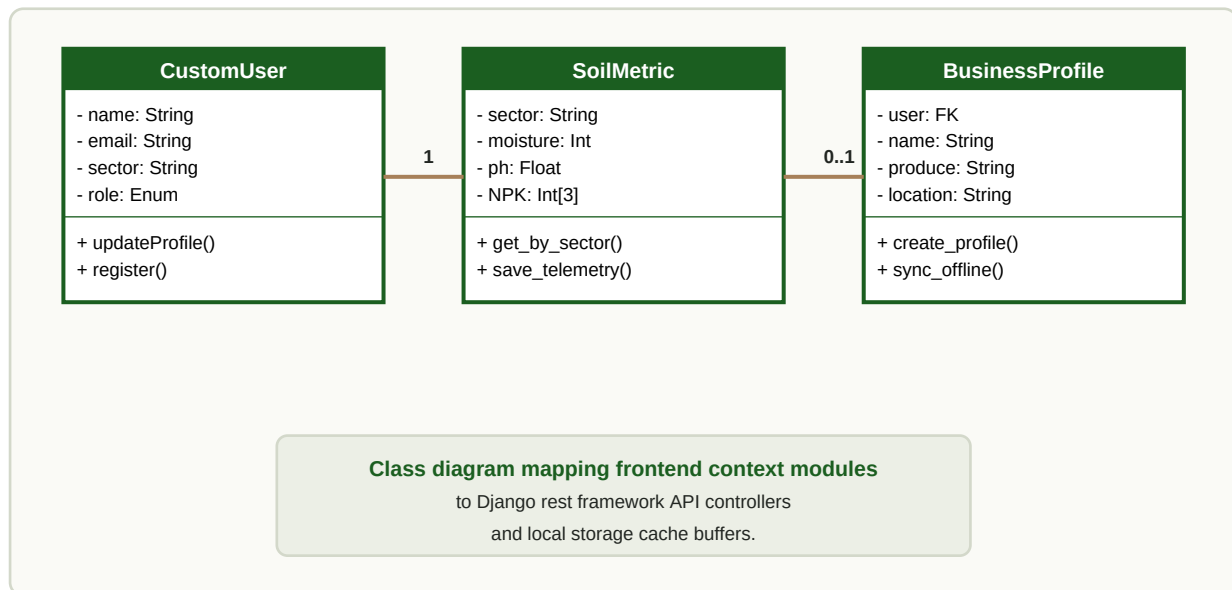
Fig 2.2.4: System Components Class Diagram
