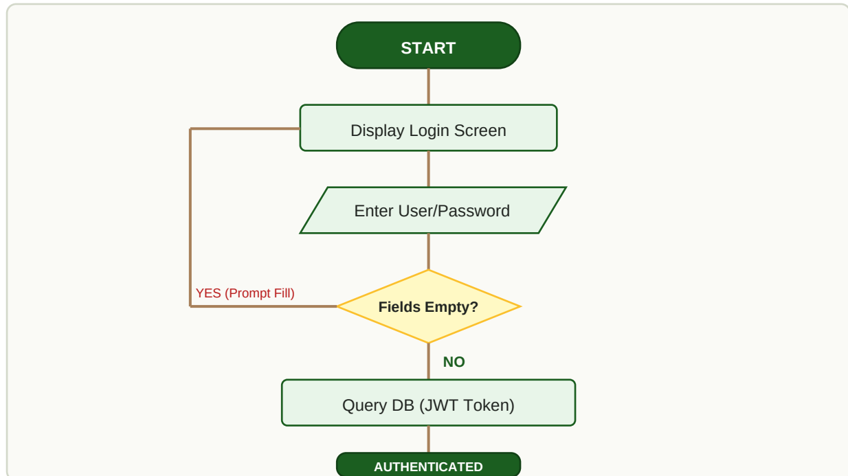
Fig 2.2.3: User Login Process Flowchart
